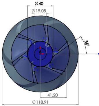
a) Digitizing the propeller in SolidWorks. b) Front view of the propeller
