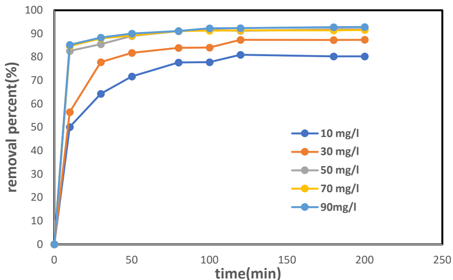
Figure 9 : Effect of Initial Concentration on CIP removal efficiency; C_0 (10-90) mg/l, particle size (424) \mu m, Temp. (25) ^{\circ} C, dosage (0.02) g/ml, pH 5, time(10-200)min. and rpm 300.
