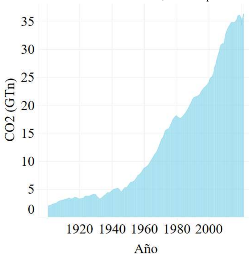
Figure 1 Amount of carbon dioxide emitted into the environment in recent years
