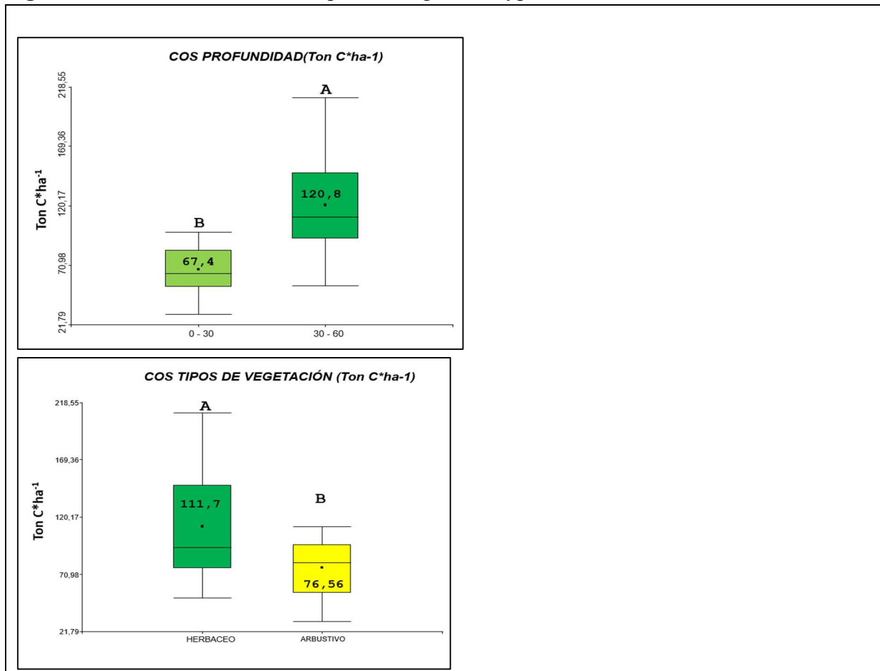
Figure 6. Carbon content at soil depth and vegetation types
